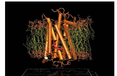
MOLECULAR DYNAMICS
