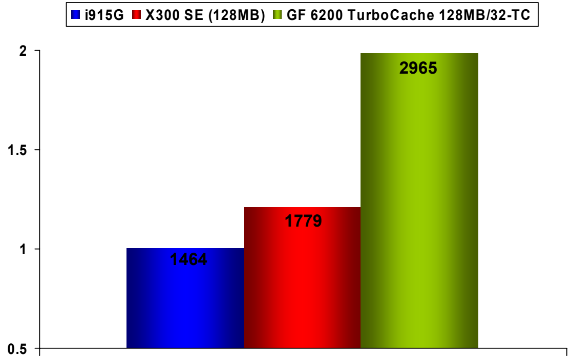
Figure 4. Graphics Performance: 3DMark03, 10 × 7, No AA or AF
