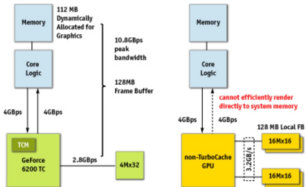
Figure 3. TurboCache Architecture vs. Non-TurboCache Architecture (for an Entry-Level PC)
